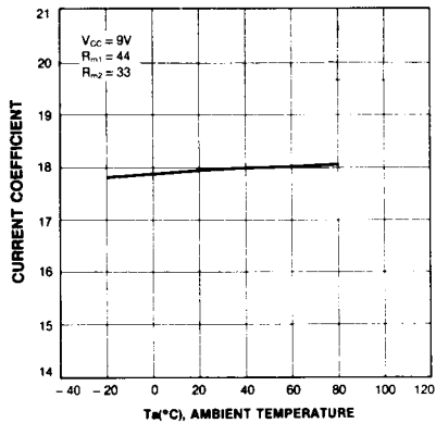
CURRENT COEFFICIENT-AMBIENT TEMPERATURE
